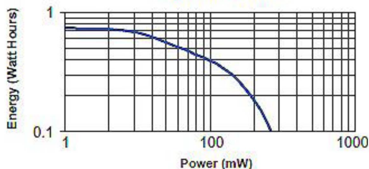
Discharge Characteristics at Various Power Drains
