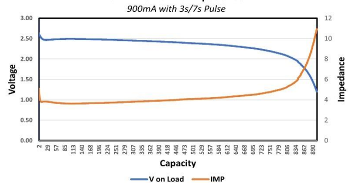
CR2 Internal DC Impedance
